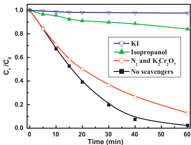
Fig. 3. The photocatalytic degradation of lamivudine without or with scavengers: [Lamivudine] = 100 μM, [TiO 2 ] = 1.00 g L -1 , and pH value 7.0.
