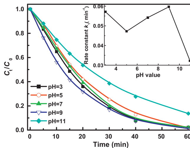
Fig. 2. Influence of pH value on the rate constants of the photocatalytic degradation of lamivudine: [Lamivudine] = 100 \mu\text{M} , and [\text{TiO}_2] = 1.00 \text{ g L}^{-1} .
