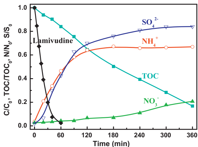
Fig. 5. Decrease of TOC and the evolution of sulphate, ammonium and nitrate ions during photocatalytic degradation of lamivudine: [Lamivudine] = 100 \mu\text{M} , [TiO 2 ] = 1.00 g L -1 , and pH value 7.0.
