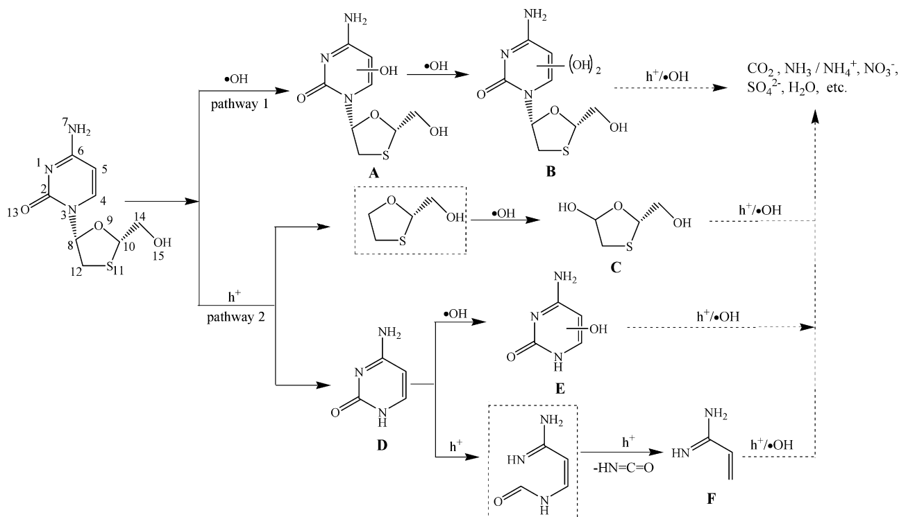
Scheme 1. Proposed photocatalytic degradation mechanism of lamivudine in \text{TiO}_2 suspension.
