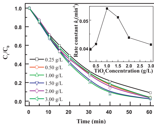
Fig. 1. Influence of \text{TiO}_2 concentration on the rate constants of the photocatalytic degradation of lamivudine: [Lamivudine] = 100 \mu\text{M} and pH value 7.0.
